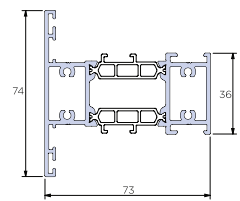
Standard Transom- Screw Fix ACW81.445
