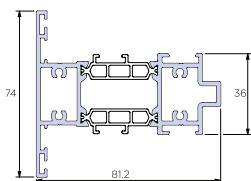
Standard Flush Transom- Screw Fix ACW81.441
