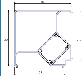
Corner Mullion ACW81.776
