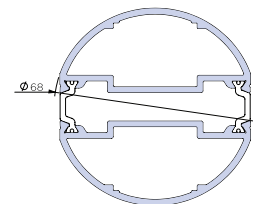
Corner Mullion ACW81.772
