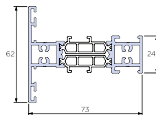
Slim Transom- Screw Fix ACW81.443
