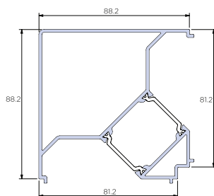
Corner Mullion ACW81.771
