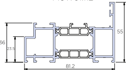
Standard Flush Outer Frame ACW81.112
