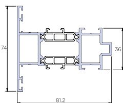
Standard Flush Transom- Cleat Fix ACW81.442
