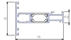
Standard Transom- Screw Fix ACW81.445
