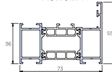
Standard Outer Frame ACW81.114
