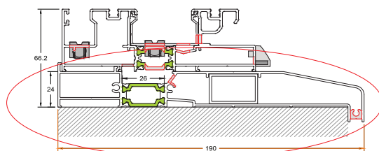
TH 80105 Sub Cill 190mm & Drainage
