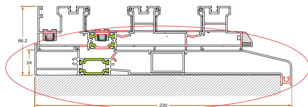
TH 80106 Sub Cill 230mm & Drainage
