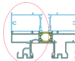
NT-80616 Detail 1 per either side of frame TH80113 or TH8022
