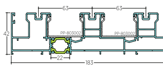
TV 12603 6,5m 1.368 gr/m Reinforcement Profile for 25mm Interlock
