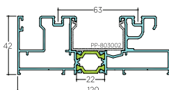
TH 8045 6,0m 1.777 gr/m Adjoining profile for Glass Sash
