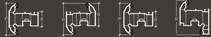
LSW031 Sash T LSW032 EnergyPlus Sash Z LSW033 EnergyPlus Sash T LSW035 T&T Sash
