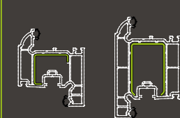
LSR035 (use with L#W035) LSR036/37 (use with L#W036/37)
