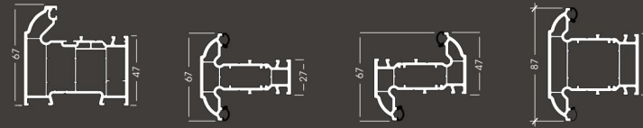
LSW018 Composite Door Outer Frame LSW021 Transom T LSW022 Transom Z LSW026 Int. Transom T
