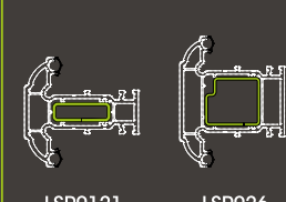
LSR021 (use with L#W021/22) LSR026 (use with L#W026)
