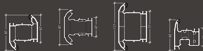
LSW027 Int. Transom Z LSW028 44mm Comp. Door Transom T LSW029 Midrail LSW030 Flush Sash
