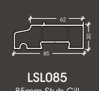
LSL085 85mm Stub Cill
