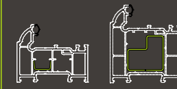
LSR011 (use with L#W011) LSR016 (use with L#W016)
