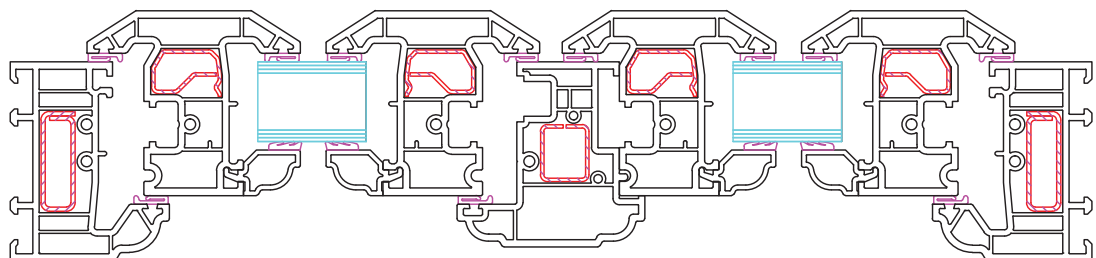
HERITAGE REBATED FRENCH CASEMENT WINDOW HORIZONTAL CROSS SECTION
