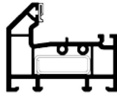
56MM PVC-U THRESHOLD (BEVELLED)
