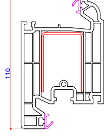
705540 (P10540) Door Sash - Open In Steel U Channel 713162 (S00162)
