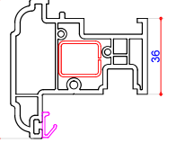
702612 (P10612) French Overlap Steel Box 713135
