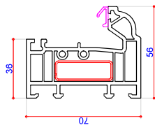
701531 (P10531) 56mm Outer Frame Steel Box 713187
