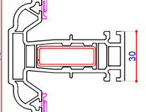
702533 70mm French Mullion Steel Box 713187 Steel Box 713155
