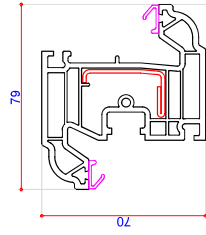
703539 (P10539) Tilt & Turn Sash Steel L Section 713161 (S00161)
