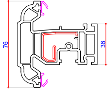
703538 (P10538) Internally Beaded Sash Steel P Section 713152 (S00152)
