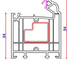
701204 84mm Outer Frame Steel P Section 713157
