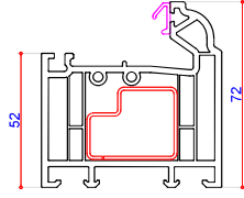
701532 (P10532) 72mm Outer Frame Steel P Section 713157
