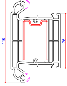
702535 (P10535) 116mm Midrail Steel U Channel 713166 (S00166)
