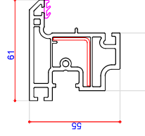
703810 Flush Sash Steel L 713226
