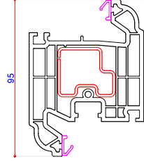
705545 (P10545) 95mm Z Transom/Slim Open In Door Sash Steel Box 713159 (S00159)
