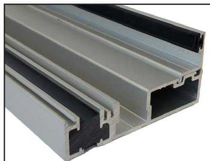
Internal Low Threshold with Rebate
