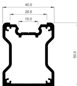
Reinforcement 40x50mm
