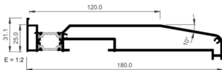
Cill 180mm
