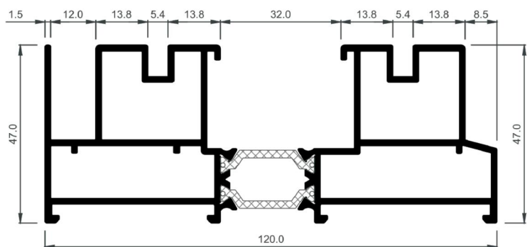
Two rail frame
