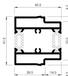
Sash joint profile
