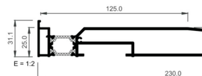
Cill 230mm
