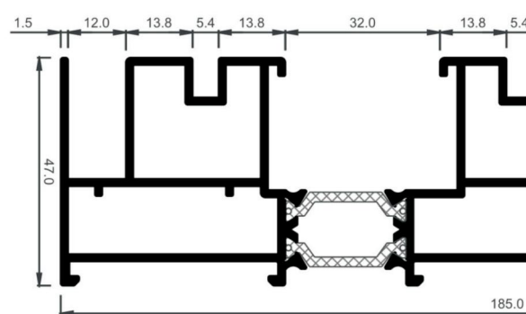
Three rail
